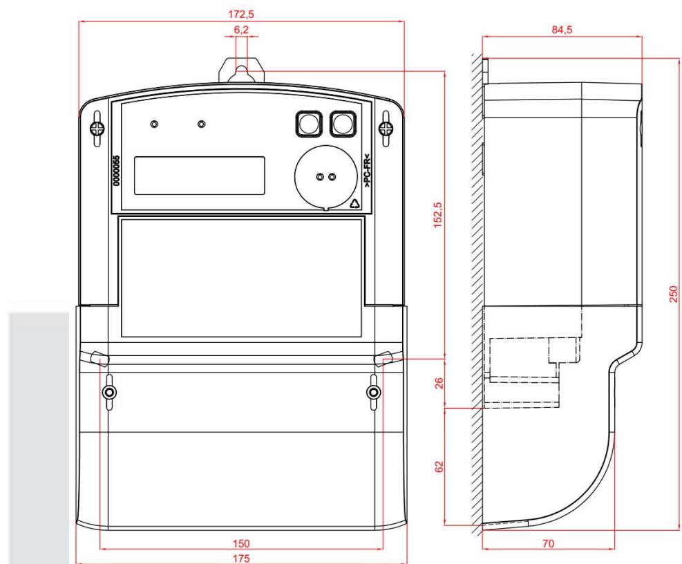
Figure 2.2. Dimensions of the meter
