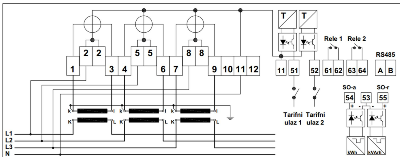
Figure 2.7 Current transformer operated meter connection scheme
