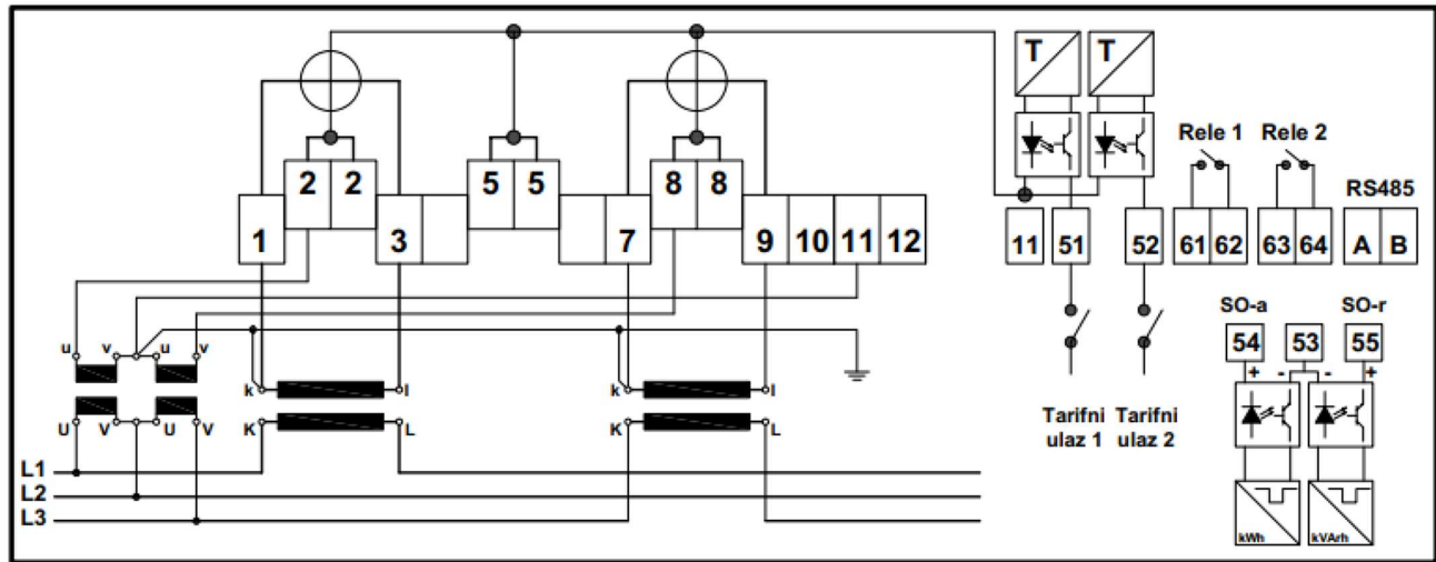
Figure 2.9 Current and voltage transformer operated meter Aaron connection scheme
