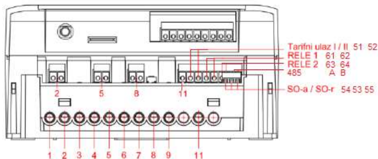
Figure 2.4 Meter terminal connector's labels (with GPRS modem)
