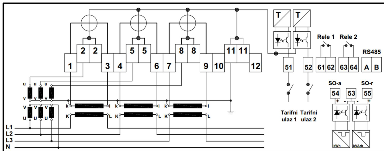
Figure 2.8 Current and voltage transformer operated meter connection scheme
