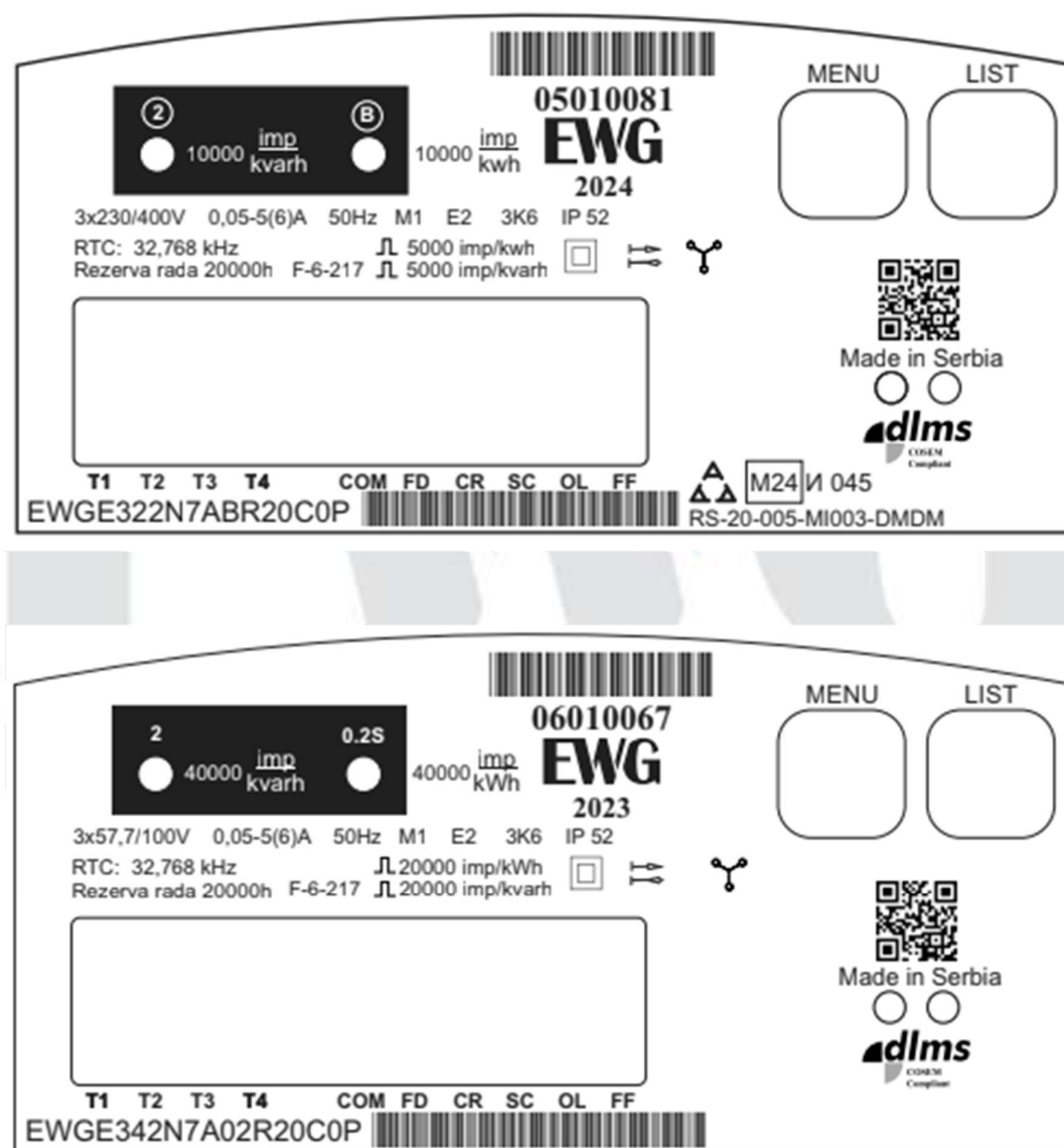
Figure 2.5 Name plates of EWGE32x and EWGE34x meters
