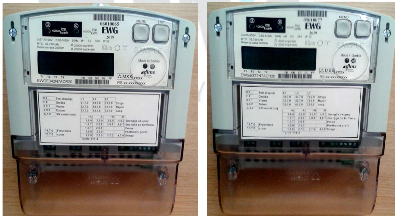
Figure 2.1 EWG meter (EWGE34x left and EWGE32x right) – front view
